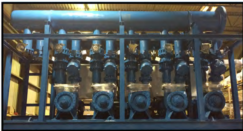
Central Heating Pumps Fort Bliss - Texas, USA
