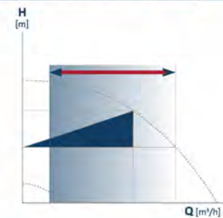
FLOWADAPT control mode
