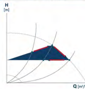
AUTOADAPT mode
