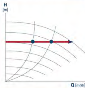
Constant pressure mode
