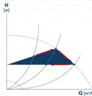
AUTOADAPT mode
