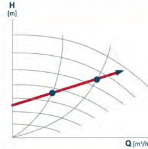
Proportional pressure mode
