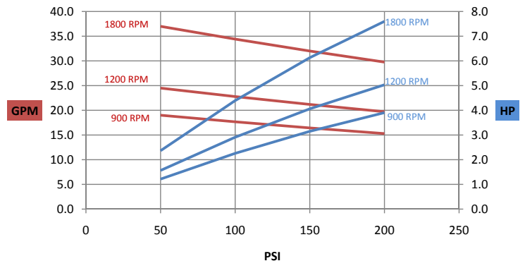
35H Pump Curves
